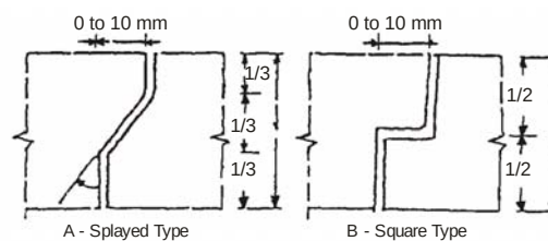
Fig. 9.16D : Meeting of Stiles for Double Leaved Door Shutters
