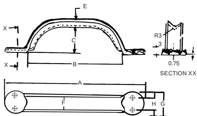
Fig. 9.12.3 : Typical Door Handle (Type 3)
