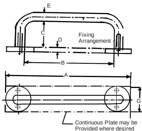
Fig. 9.12.3 : Typical Door Handle (Type 3)
