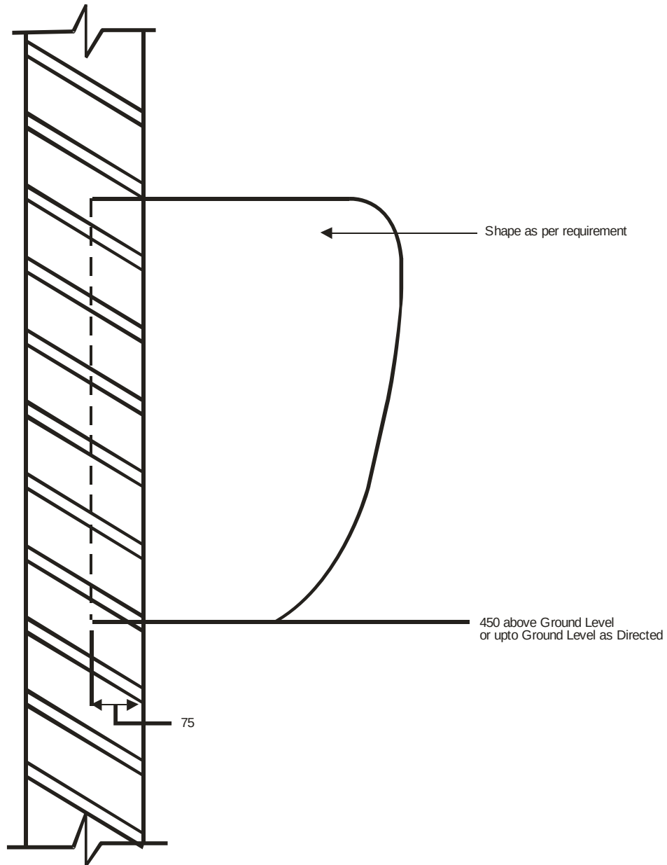
Fig. 8.4 : Marble Slab Urinal Partition
